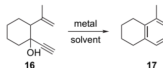
Scheme 2. Metal-mediated benzannulation.
