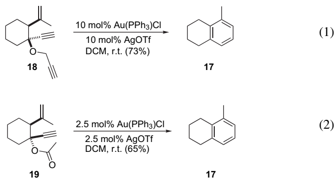
Scheme 3. Benzannulation of enynes.
