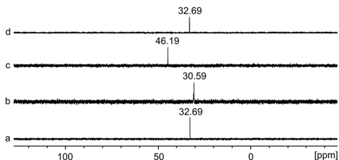
Figure 2. ^{31}\text{P} NMR study at 23 °C in \text{CDCl}_3 ( \text{PPh}_3 used as a standard at -6.0 ppm). (a) \text{Au}(\text{PPh}_3)\text{Cl} ; (b) \text{Au}(\text{PPh}_3)\text{Cl} (2.5 mol %) and \text{AgOTf} (2.5 mol %) after 16 h; (c) \text{Au}(\text{PPh}_3)\text{Cl} (2.5 mol %), \text{AgOTf} (2.5 mol %), and alcohol 16 (59% conversion); (d) \text{Au}(\text{PPh}_3)\text{Cl} (5 mol %), \text{TfOH} (5 mol %), and alcohol 16 (37% conversion).
