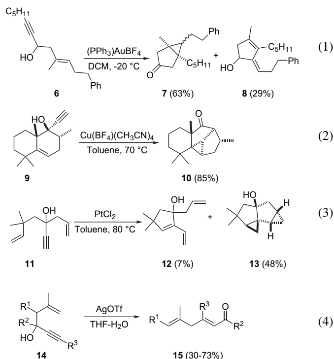
Scheme 1. Metal-catalyzed rearrangement of hydroxy-enynes.
