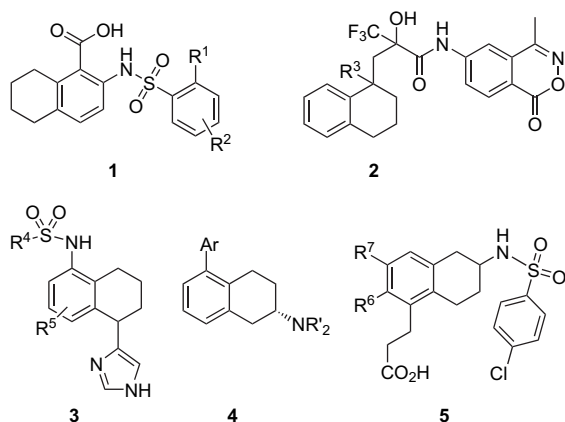
Figure 1. Examples of biologically active tetrahydronaphthalenes.
