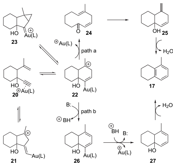
Scheme 4. Proposed mechanism for Au(I)-catalyzed benzannulation.
